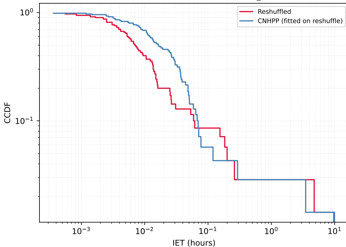
User 5229698385 - Reshuffled vs CNHPP A_{\text{fit}}=0.6146
